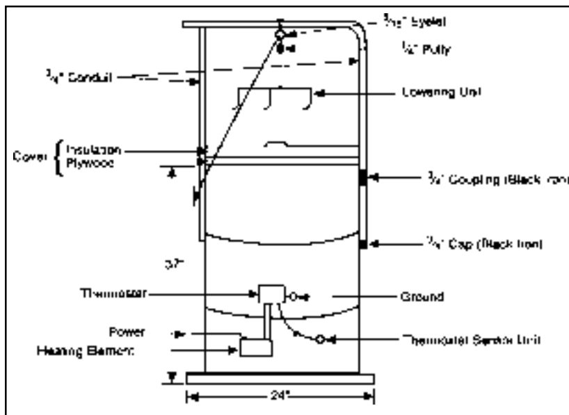
Fig 4. View of completed boiling apparatus.
