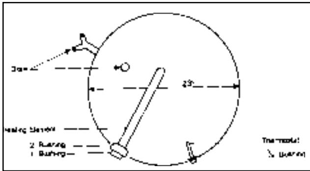
Fig 2. Top view of boiling apparatus.
